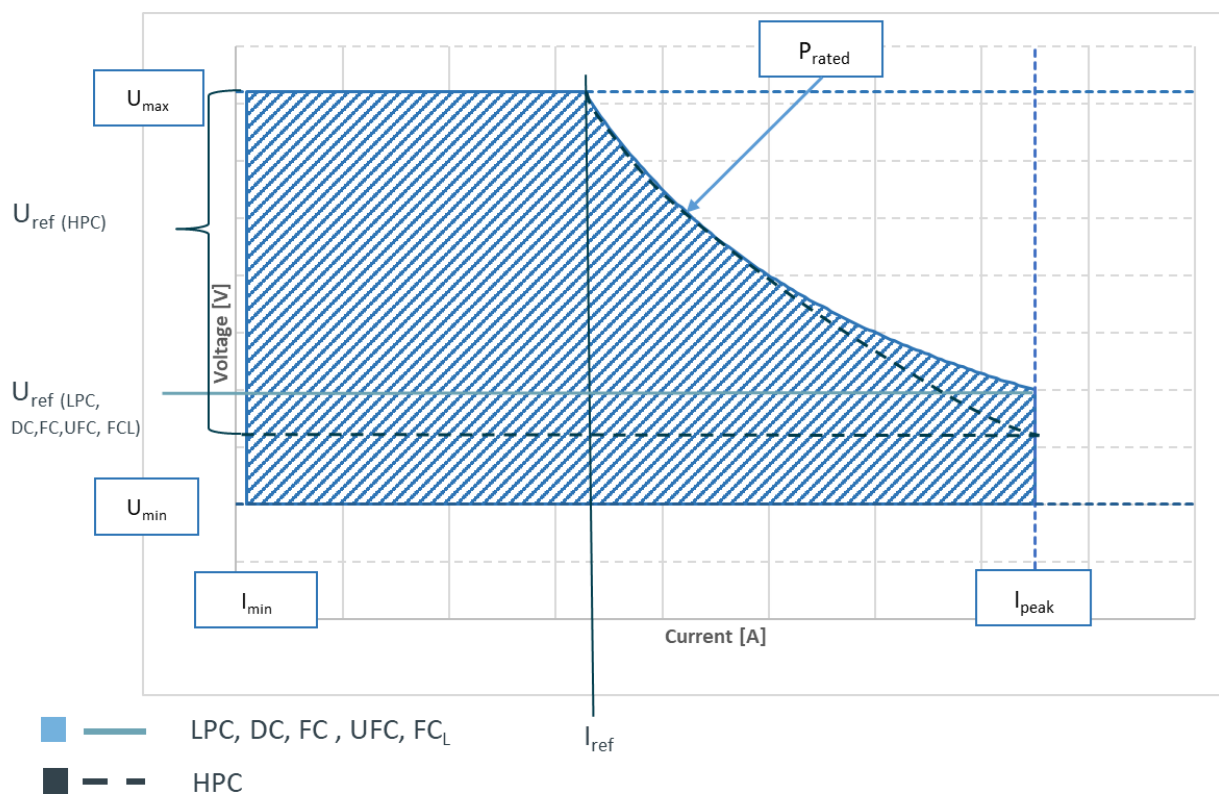
Figure 1 power class range diagram
